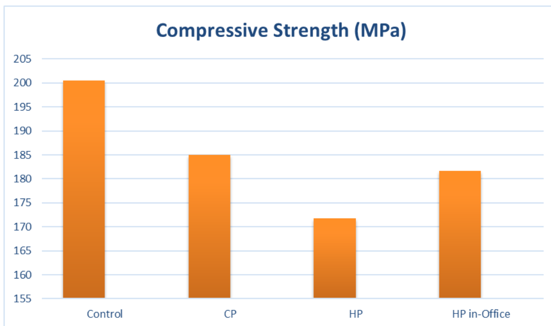
Figure 11 : Bar Chart of compressive strength of all groups.
